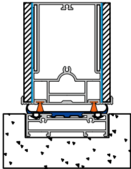
Recessed Threshold Κρυφό Κατωκάσι Soglia nascosta
